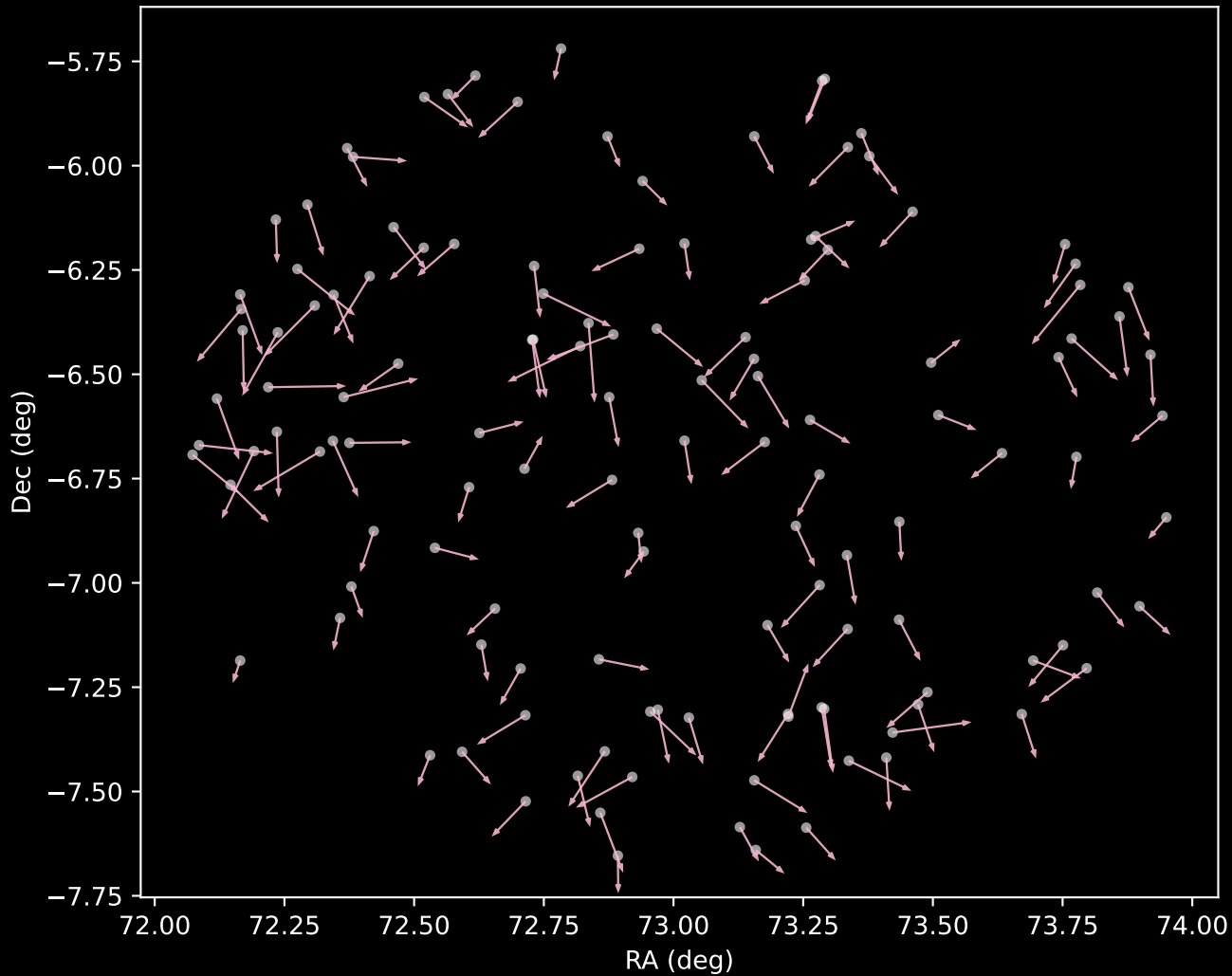
GALAH DR4 Cluster 13 Proper Motion Vectors (n=131)
