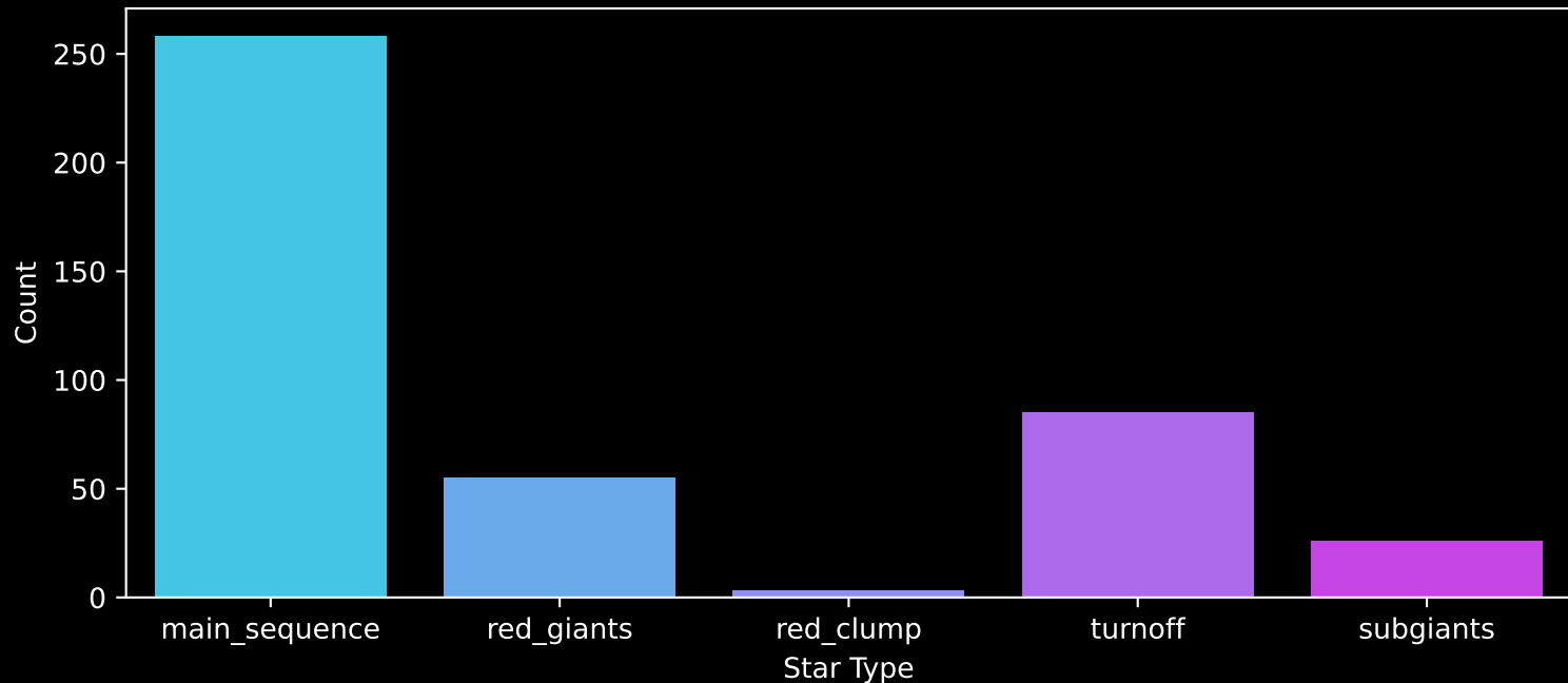
GALAH DR4 Field: [6575] Count plot of Star Type
