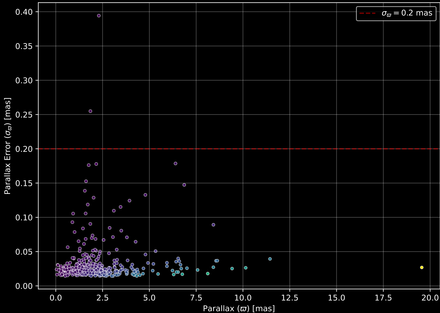
GALAH DR4 Field: [6575] Parallax Quality (n= 427)
