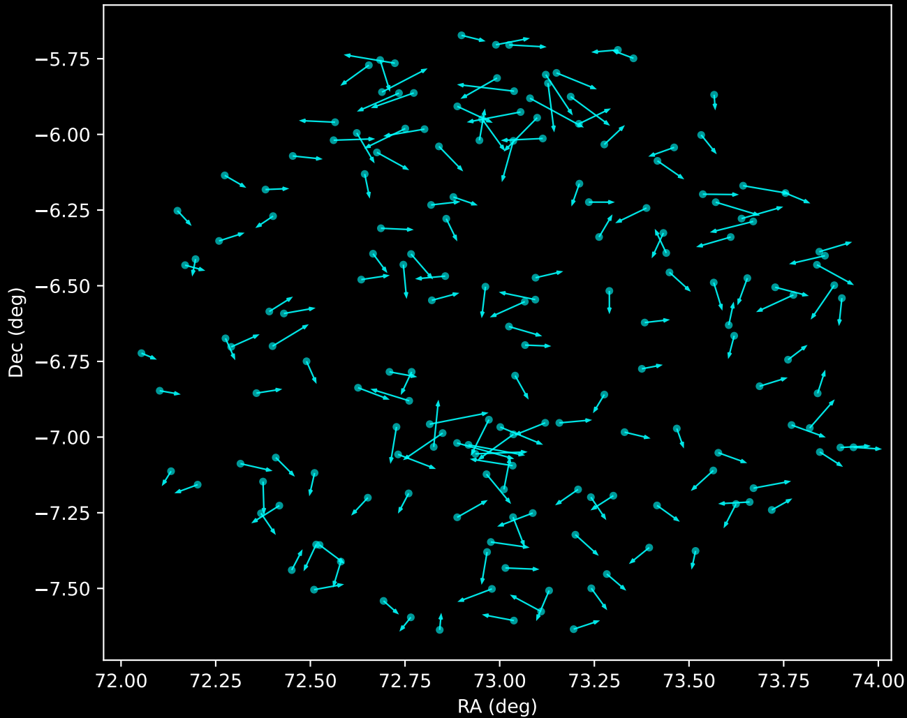
GALAH DR4 Noise Stream Proper Motion Vectors (n=176)
