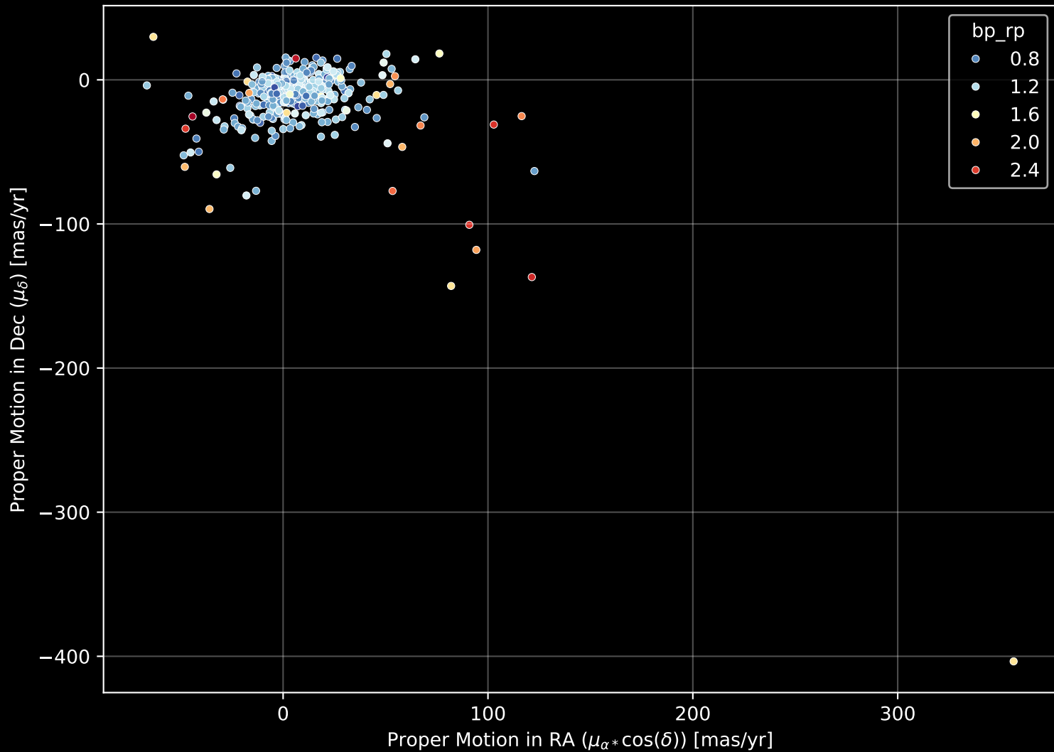
GALAH DR4 Field: [6575] Proper Motion Diagram (n= 427)
