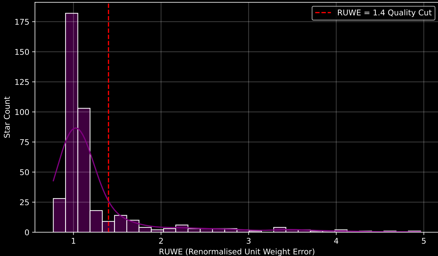
GALAH DR4 Field [6575] RUWE Distribution (n= 409)
